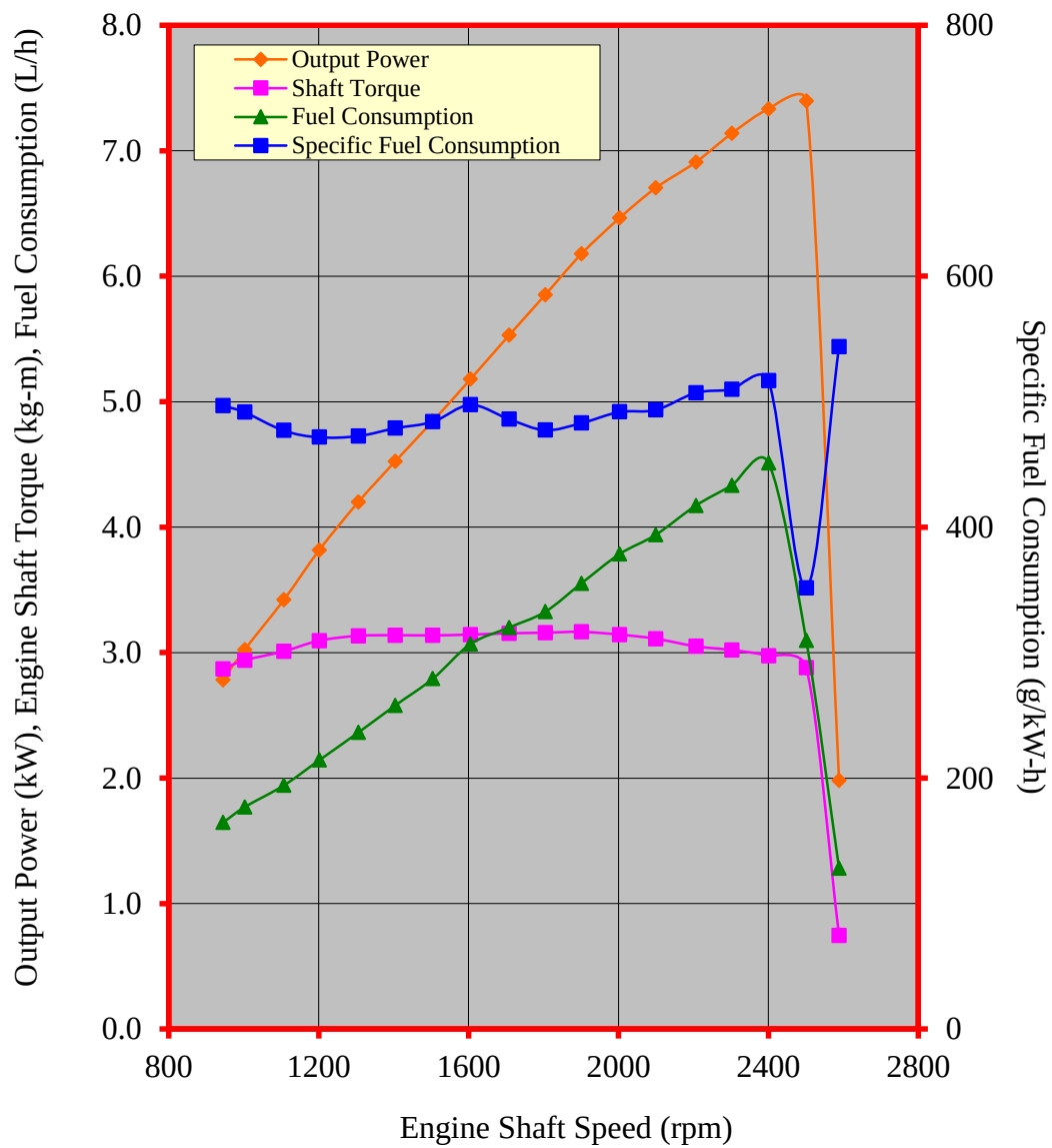
Figure 3. Performance characteristic curves of the KUTHAICO KS95B Plus Diesel Engine
