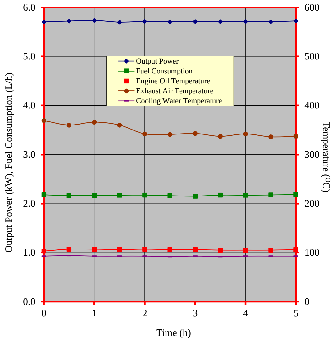
Figure 4. Performance characteristic curves during the continuous running test of the KUTHAICO KS95B Plus Diesel Engine
